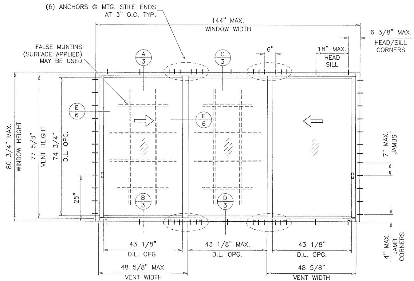
TYPICAL ELEVATIONS EQUAL LITES
