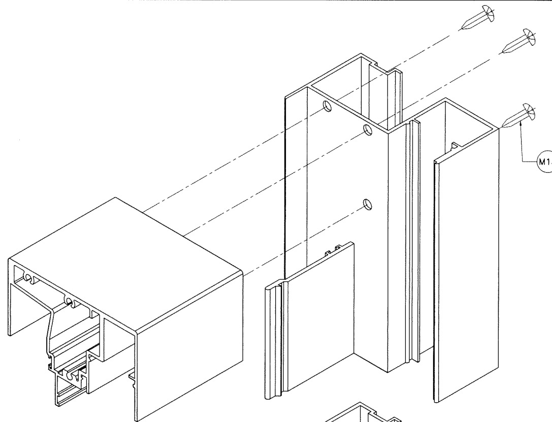
FRAME TOP CORNER
