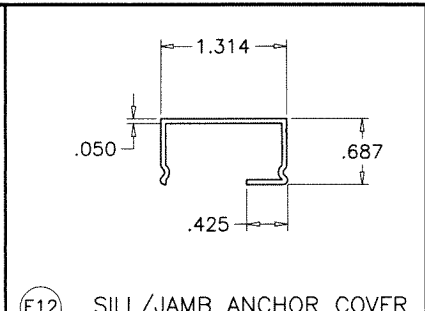
(E12) SILL/JAMB ANCHOR COVER
